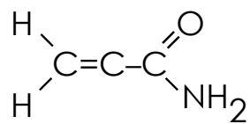
Acrylamide
